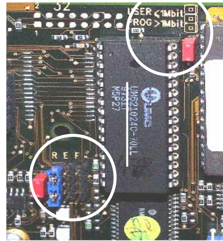
Memory jumpers in a PCD2.M120 equipped with LM621024 memory
